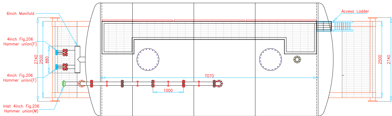
PLAN VIEW
